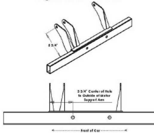
Legends Left Side Motor Mount
